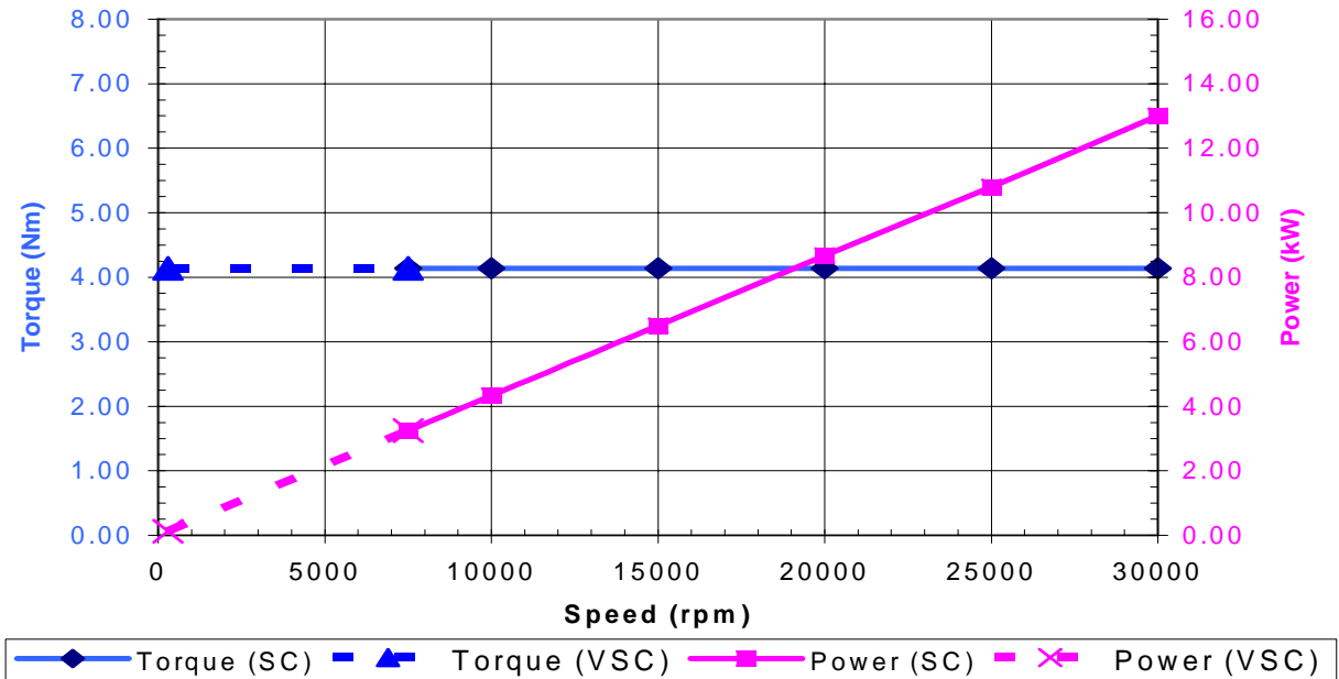
SC 60121 and VSC 60121 Power / Torque Curves (S1-100%)
